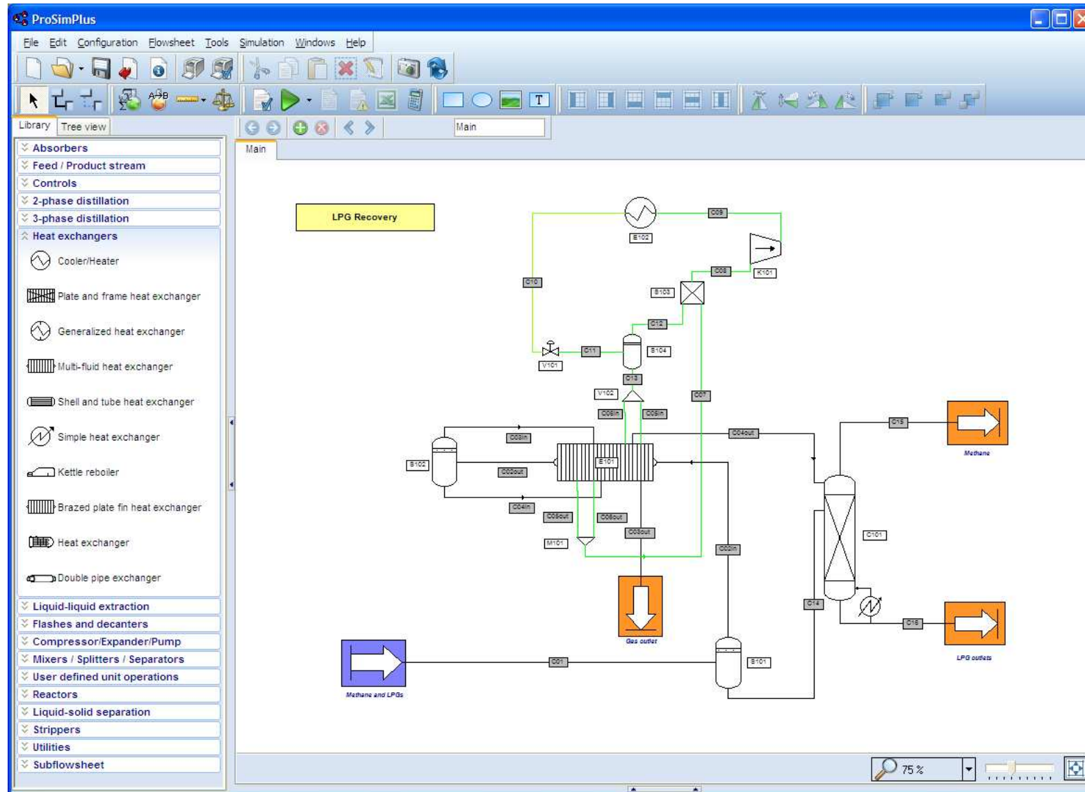
LPG recovery unit process flowsheet
